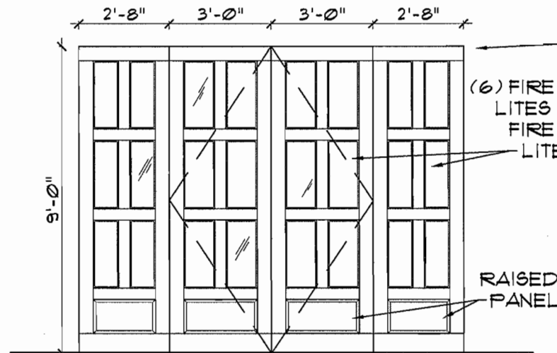
(E) SANCTUARY DOORS
