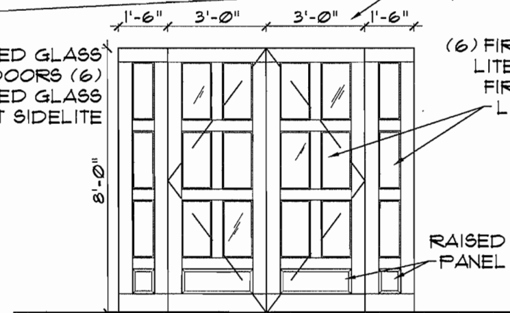
(F) SANCTUARY DOORS
